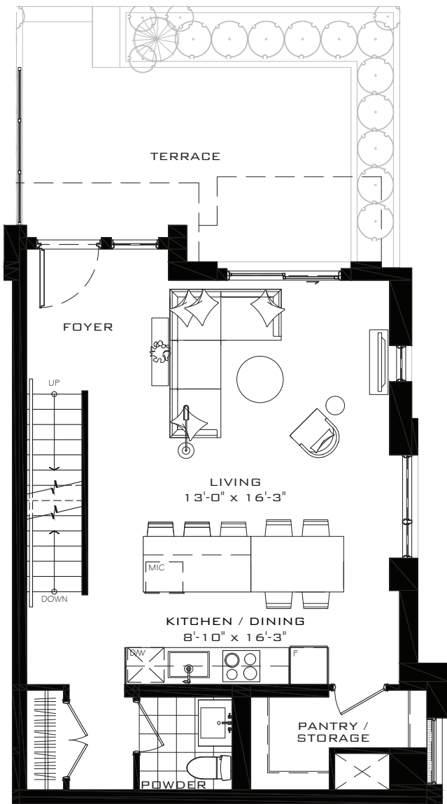
TOWNHOUSE 01 GROUND FLOOR - 634 SQ. FT.
