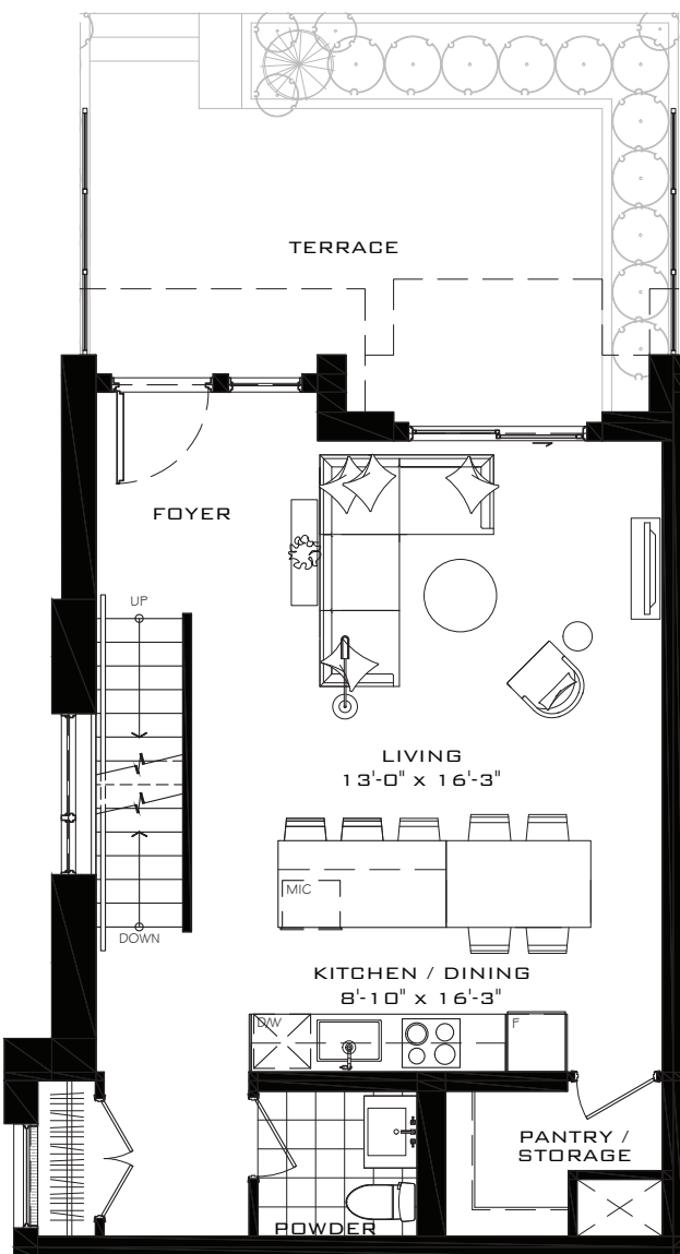
TOWNHOUSE 07 GROUND FLOOR - 637 SQ. FT.
