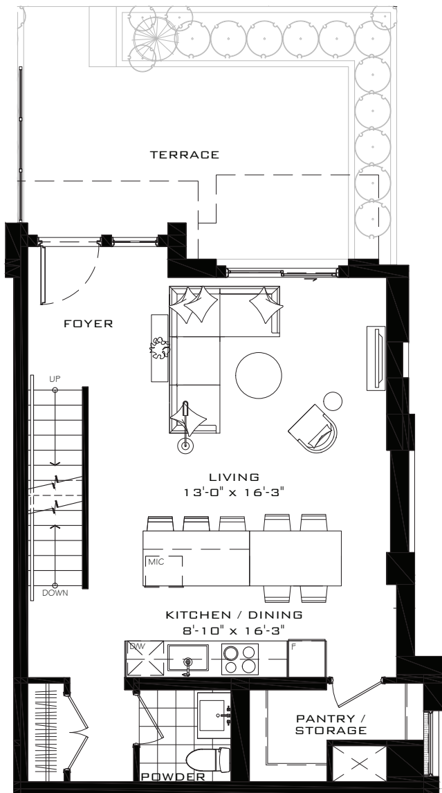
TOWNHOUSE 08 GROUND FLOOR - 634 SQ. FT.
