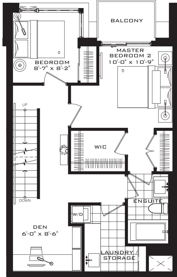
TOWNHOUSE 09, 10, 11, 12, & 13 SECOND FLOOR - 621 SQ. FT.
