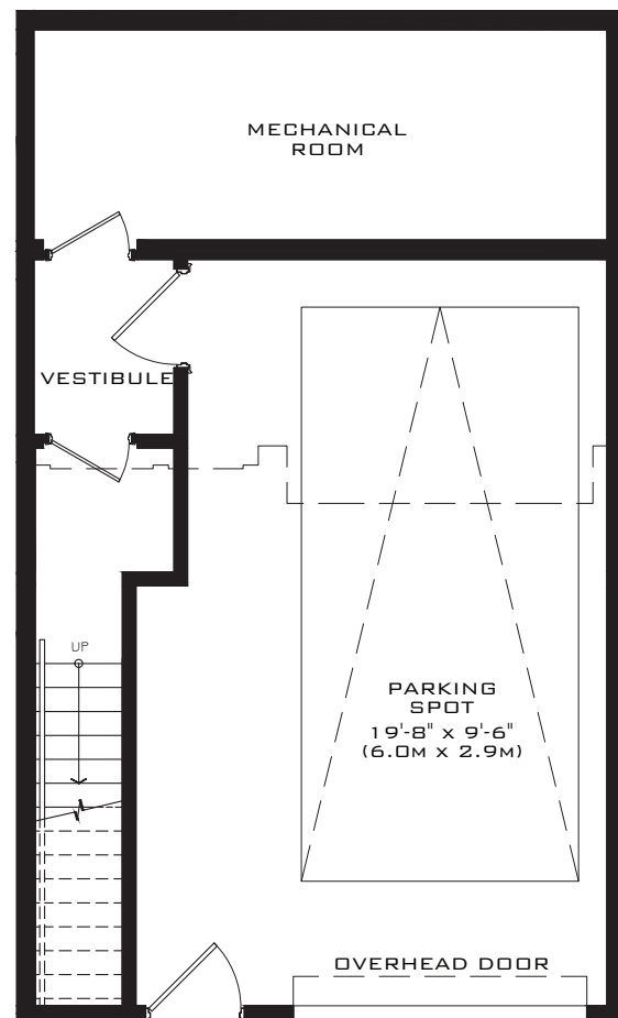
TOWNHOUSE 09, 10, 11, 12, & 13 BASEMENT - 703 SQ. FT.
