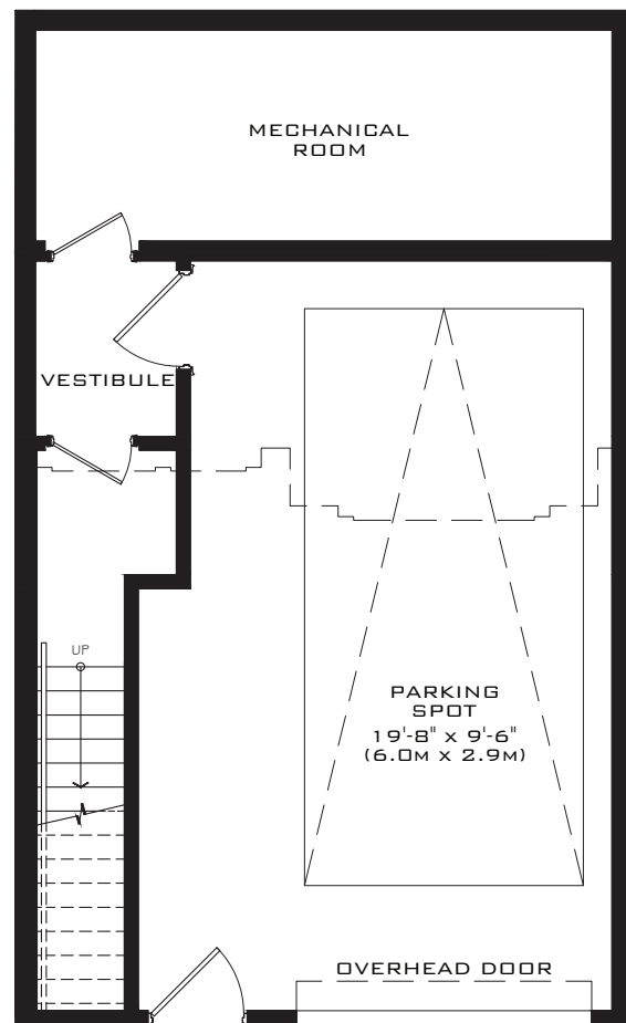
TOWNHOUSE 14 BASEMENT - 715 SQ. FT.
